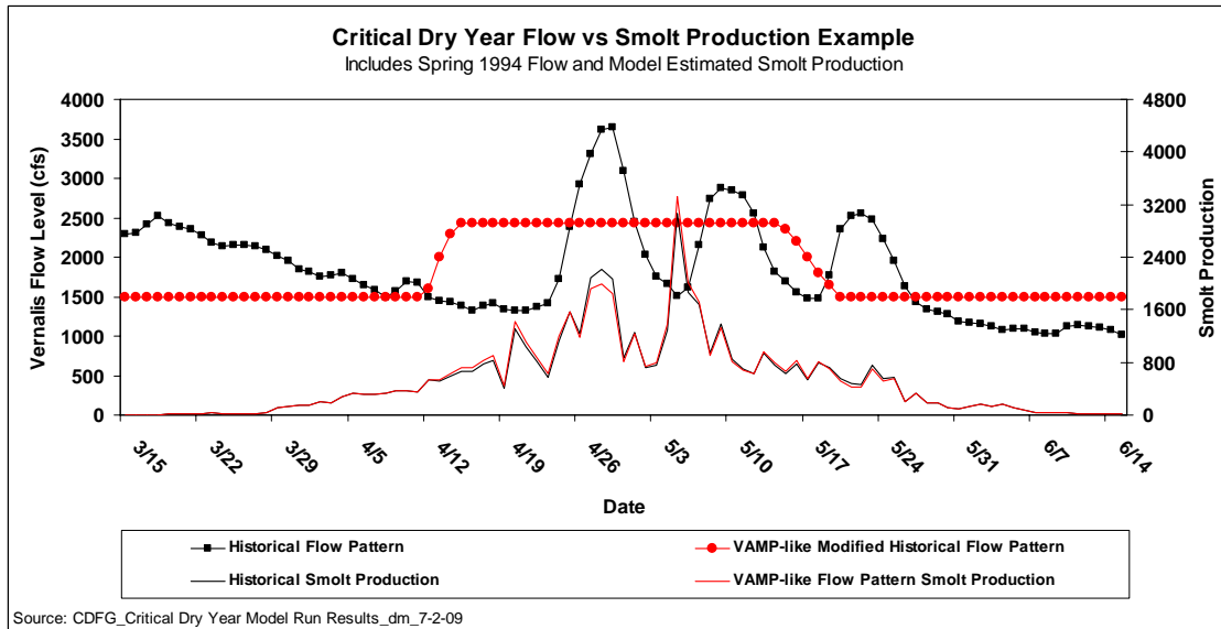
Figure 7 Critically Dry Year Example-Changing Historical Flow to VAMP-like Flow
